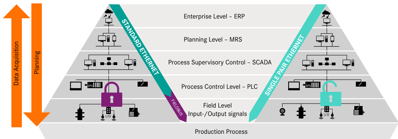
Figure: The change in the industrial network due to Single Pair Ethernet
