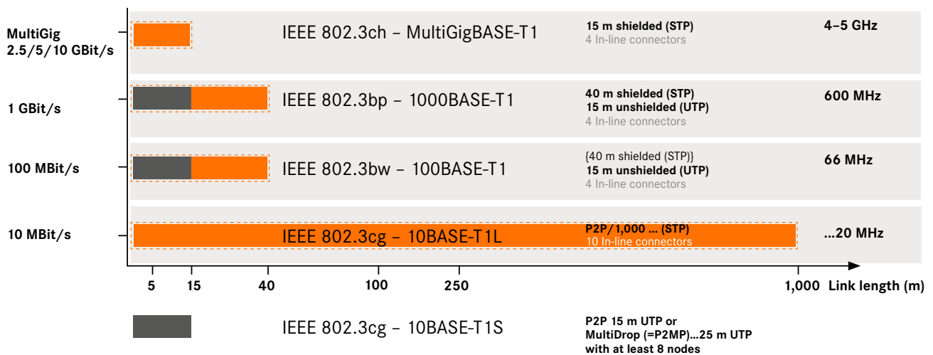
Figure: Overview of the IEEE protocol standards for Single Pair Ethernet
